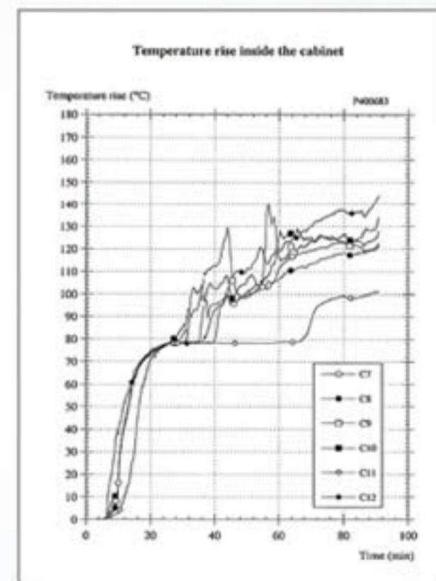
● Heat Graph (C7-12)
