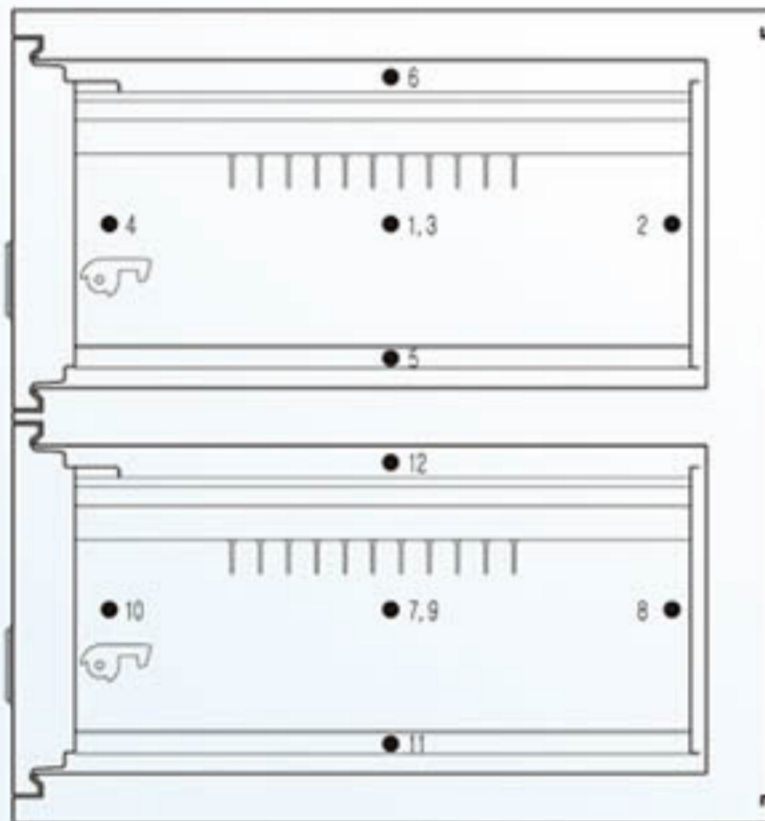
● Location of Thermocouples
