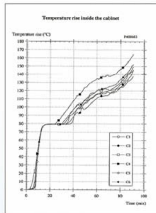
● Heat Graph (C1-6)
